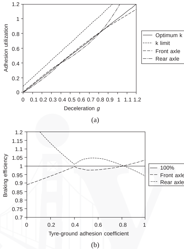
Figure 14.21 (a) Adhesion utilization, modified vehicle fitted with deceleration sensitive pressure modulating valve, (b) brake system efficiency, modified vehicle fitted with deceleration sensitive pressure modulating valve
