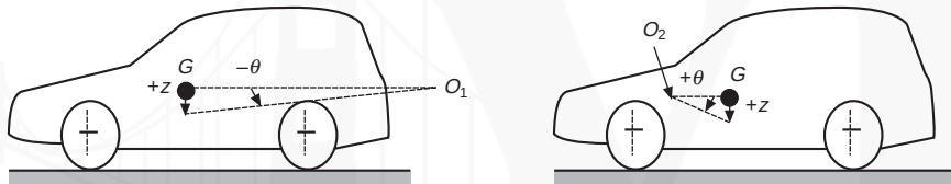
Figure 10.50 Location of oscillation centres
