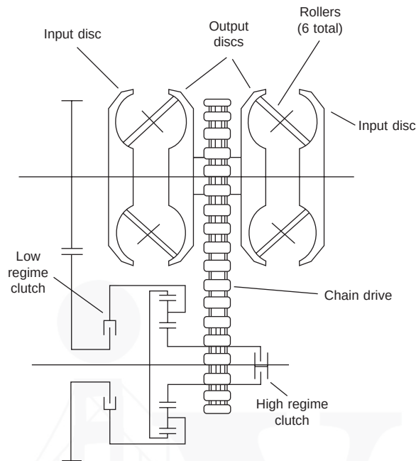
Figure 13.33 Torotrak transmission schematic layout
