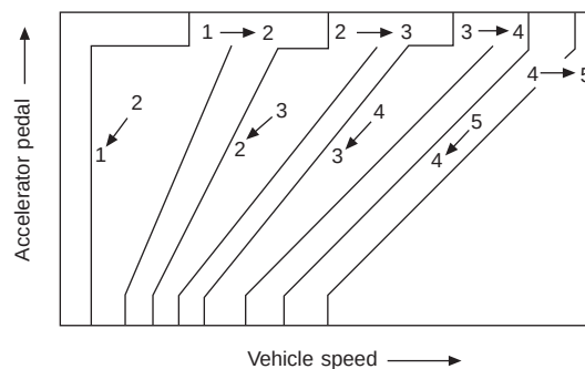
Figure 13.23 Shift strategy (courtesy of Jatco)
