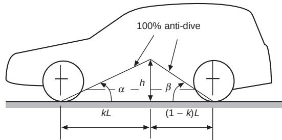
Figure 10.32 Suspension pivot locii for 100% anti-dive during braking (outboard brakes)
