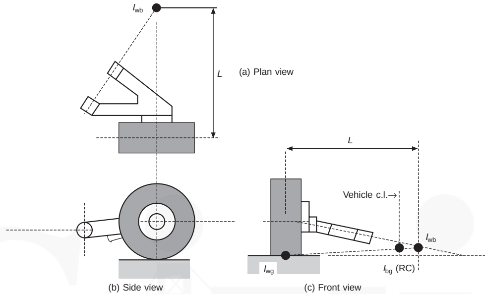
Figure 10.21 Roll centre location for semi-trailing arm suspension
