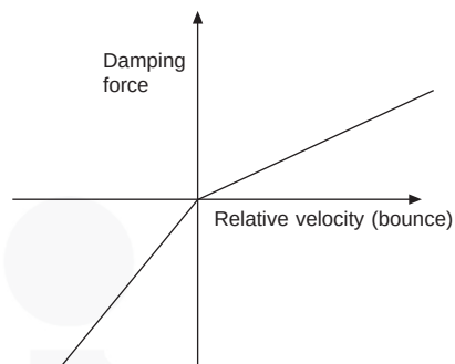
Figure 10.41 Non-linear damper characteristics
