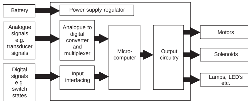
Figure 11.7 Microcomputer-based electronic control unit
