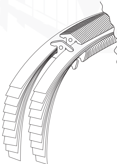
Figure 13.28 The Van Doorne metal belt construction
