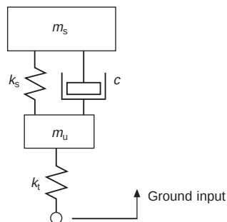
Figure 8.2 Quarter vehicle suspension model
