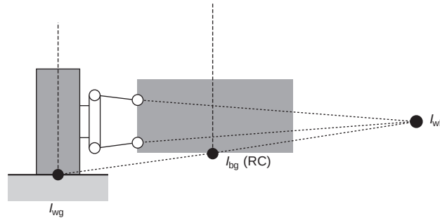
Figure 10.17 Roll centre determination for double wishbone suspension
