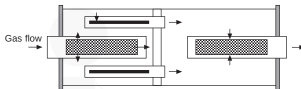
Figure 8.26 Two-chamber reactive silencer
