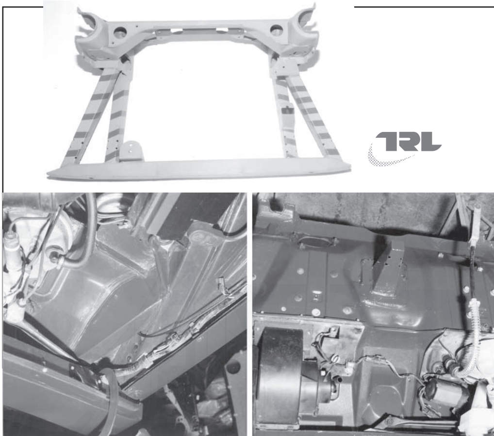
Figure 7.14 Engine subframe with front beam and energy absorbing tubes, box section triangulation and firewall energy absorber
