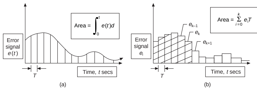
Figure 11.5 Continuous and sampled error signal levels showing digital integration (Bissel, 1992)
