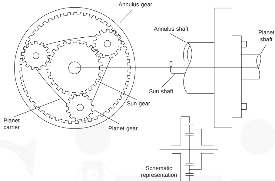
Figure 13.20 An epicyclic gear and stick equivalent
