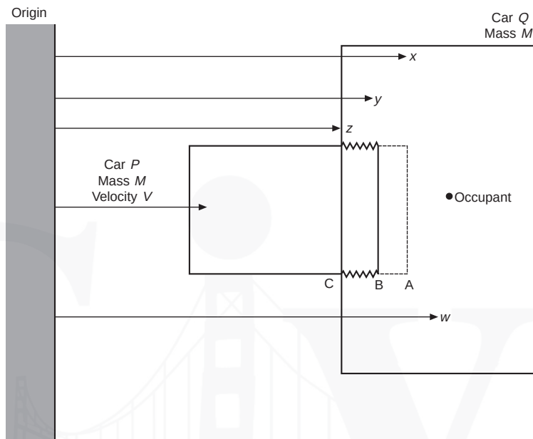
Figure 7.8 A representation of a side impact
