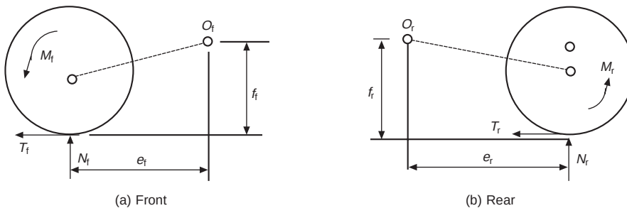
Figure 10.33 Wheel forces and effective pivot locations
