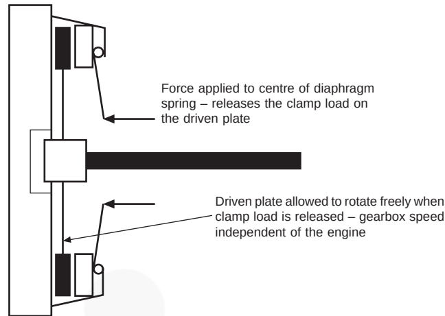
Figure 13.14 Diagram of clutch when released
