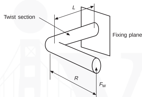
Figure 10.37 Principle of operation of a torsion bar spring
