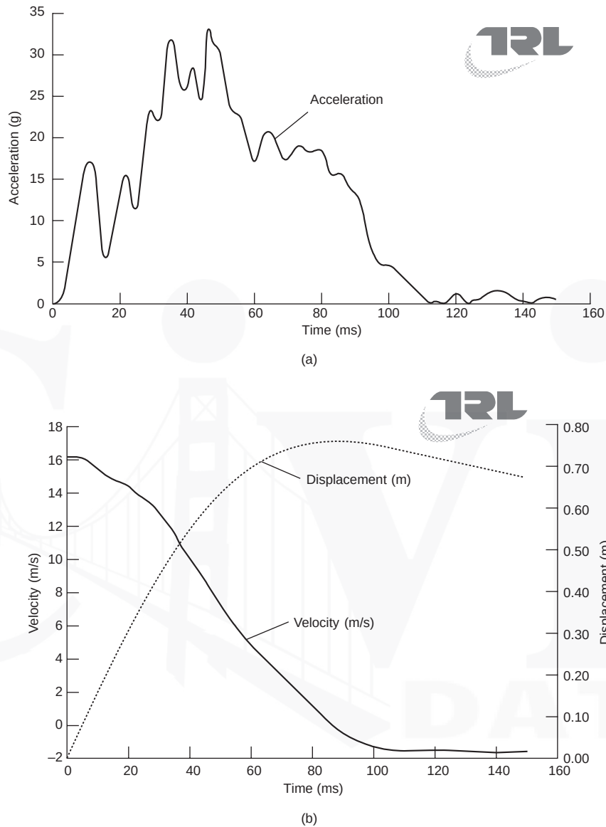
Figure 7.4 (a) Acceleration against time of an impact of a Vauxhall Cavalier at 58 km/h into a rigid barrier (b) Velocity and displacement against time of the impact shown in Figure 7.4(a)
