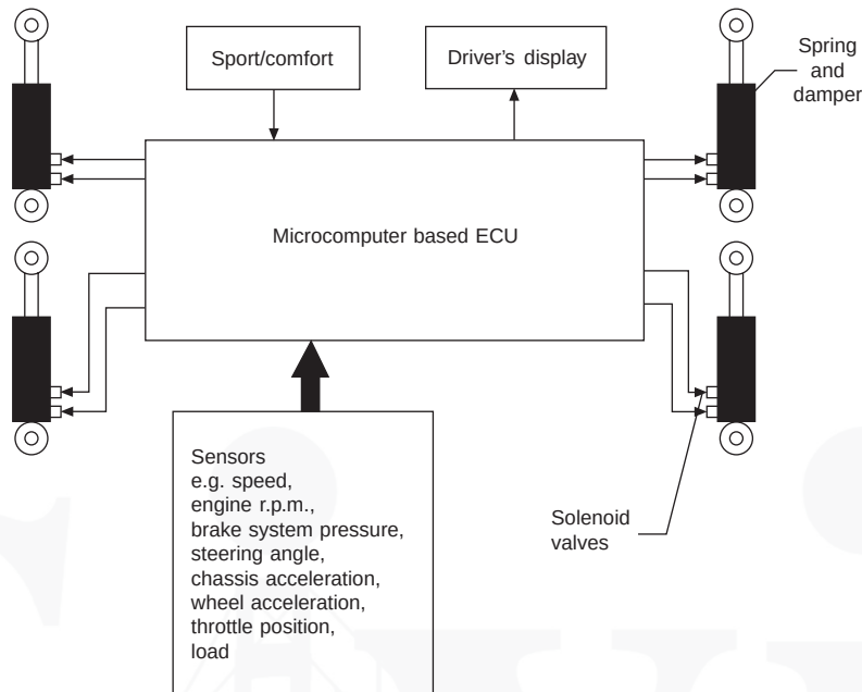
Figure 11.23 Electronically controlled damping system (Chowanietz, 1995)
