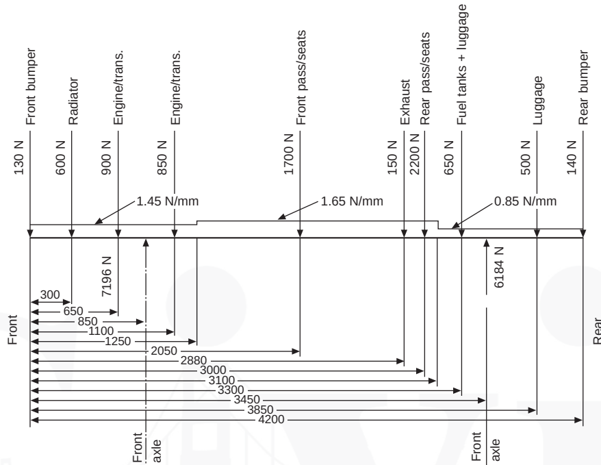
Figure 6.2 Typical passenger vehicle bending loads
