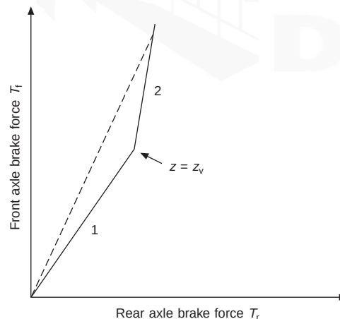
Figure 14.20 Typical modulating valve brake force distribution
